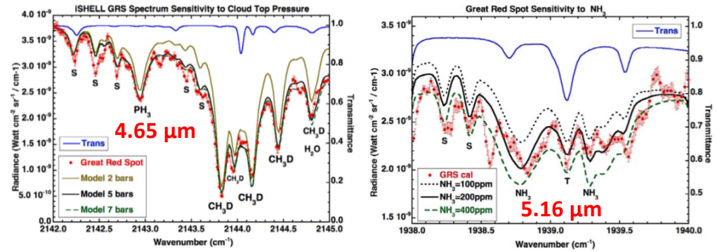
Selection of iSHELL spectra ( R=40,000 )
