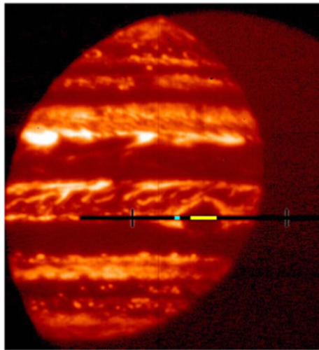
5.1 \mu\text{m} slit-viewer image
