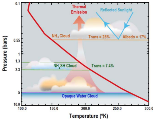
Great Red Spot cloud model from iSHELL data
