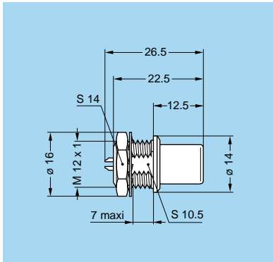
FAA Fixed plug, nut fixing, non-latching
