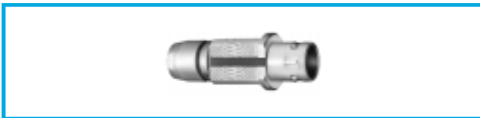
FIG Straight plug for remote handling, key (G) or keys (A...L and R), special alignment mark, knurled handling surface, cable collet
