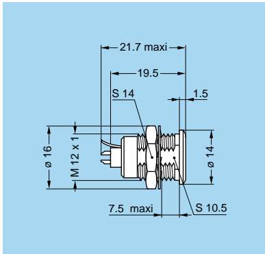
ERN Fixed socket nut fixing, with earthing tag
