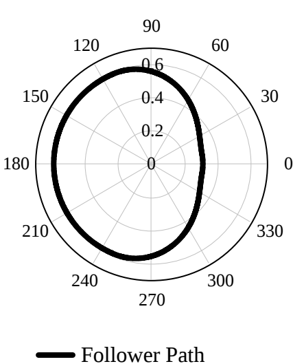
Cam Follower Path
