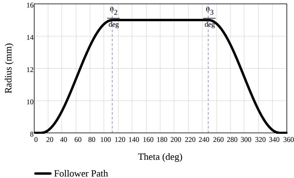
Cam Follower Path vs. Follower Angle
