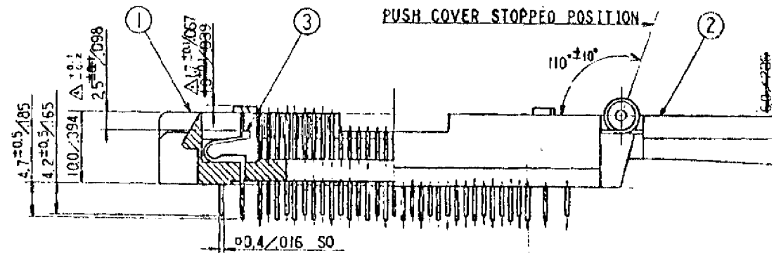
SECTION X-X
