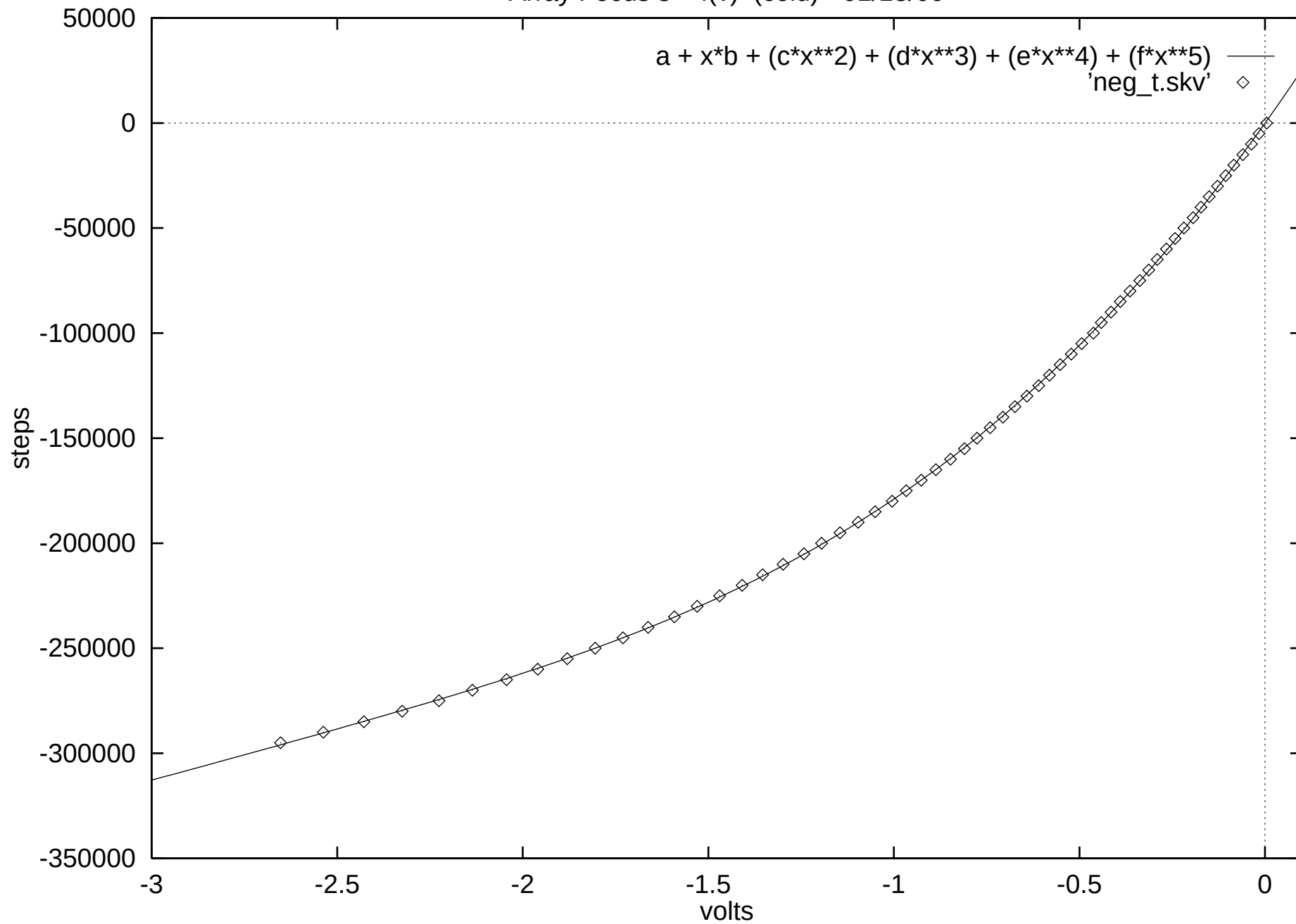
Array Focus s = f(v) (cold) - 01/13/00
