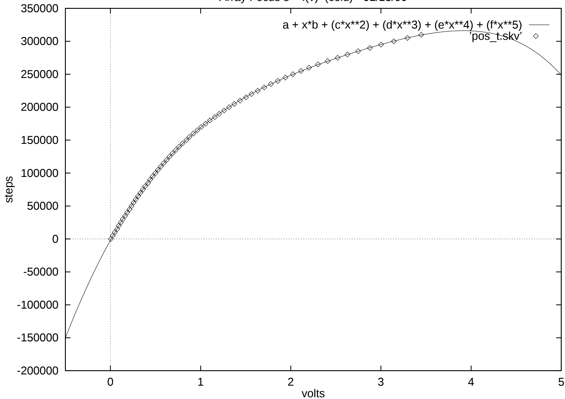
Array Focus s = f(v) (cold) - 01/13/00
