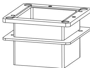
ISOMETRIC SCALE 1/2
