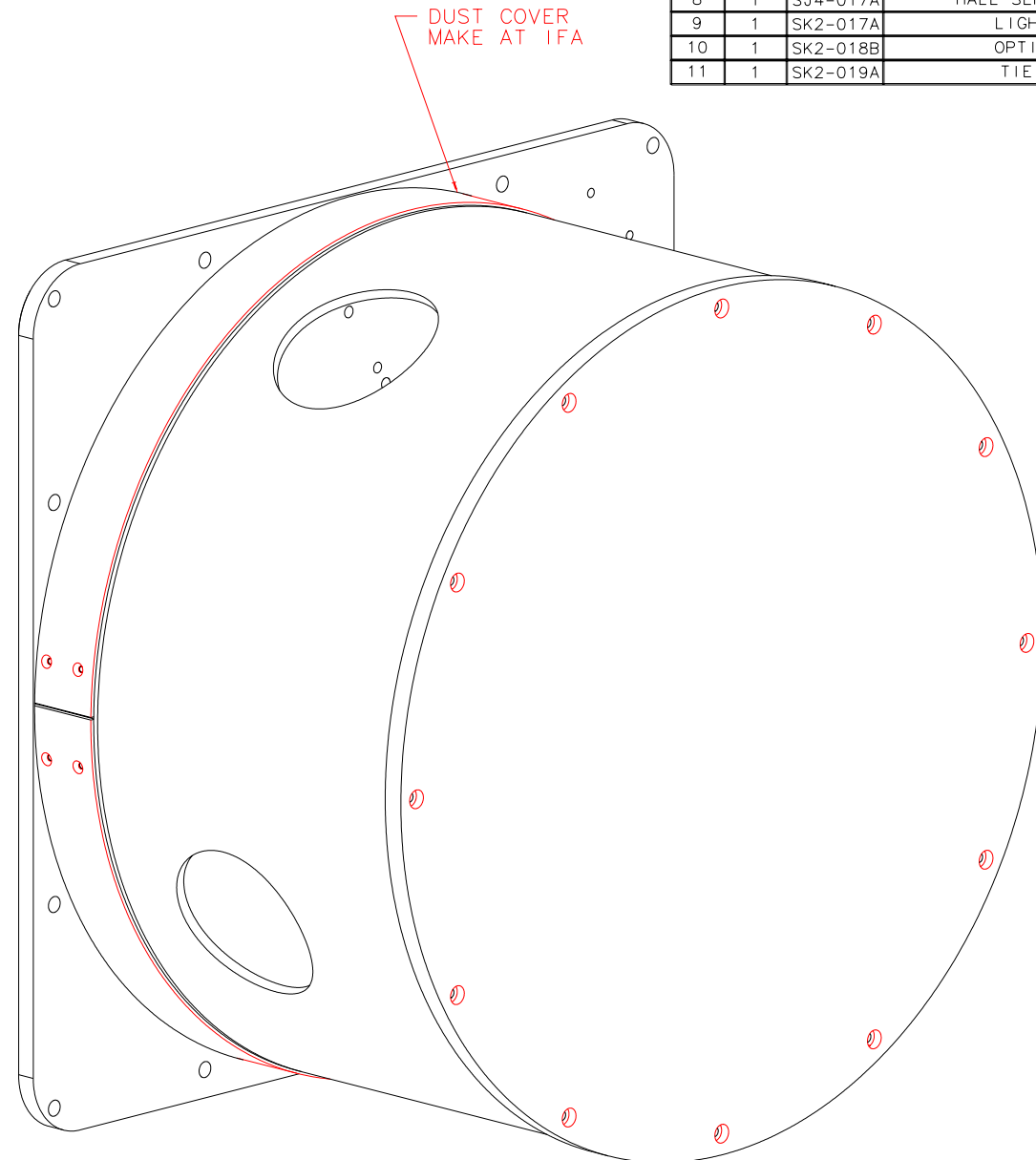
ISOVIEW 2 SCALE 1:2
