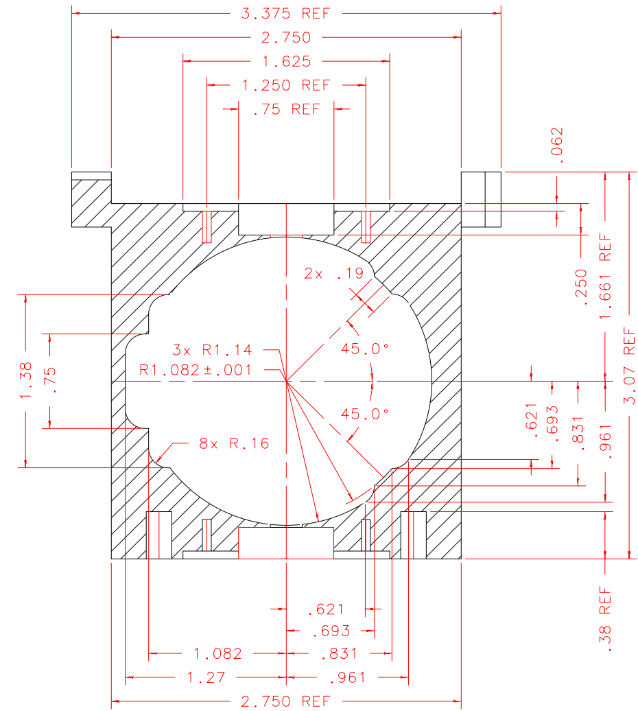
SECTION B-B
