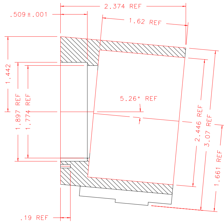
SECTION B-B
