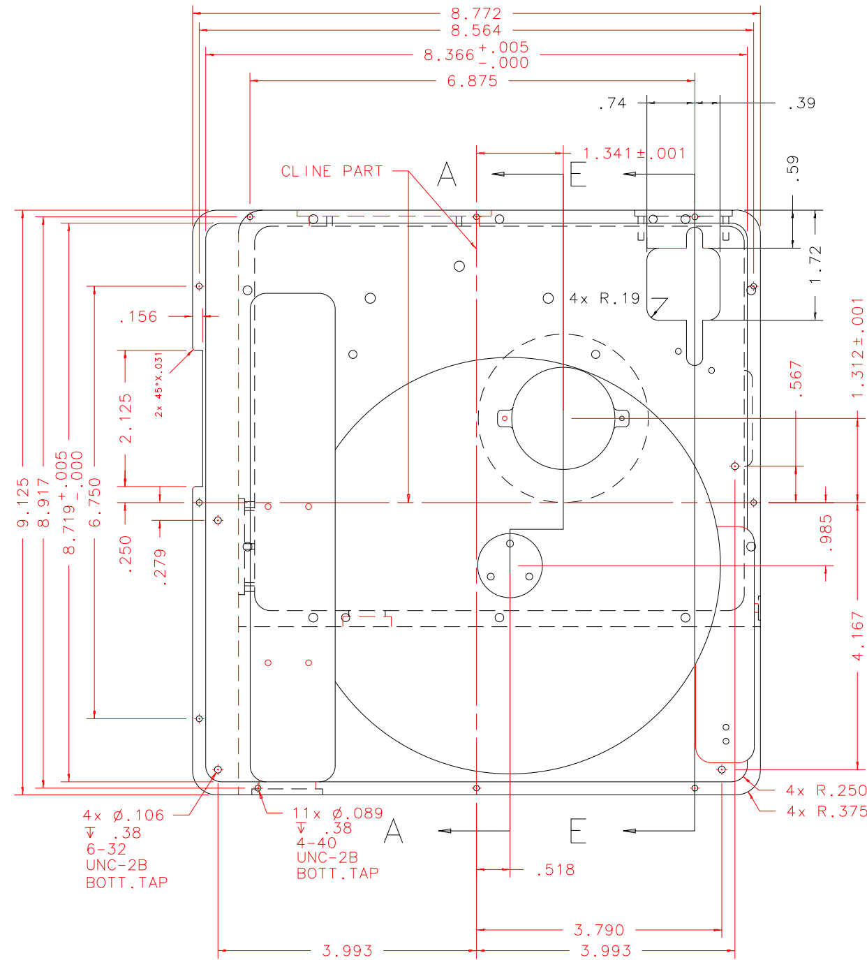
FRONT: SCALE 1:2 SEE ALSO SHEET 6&7 FOR DUPLICATE VIEW
