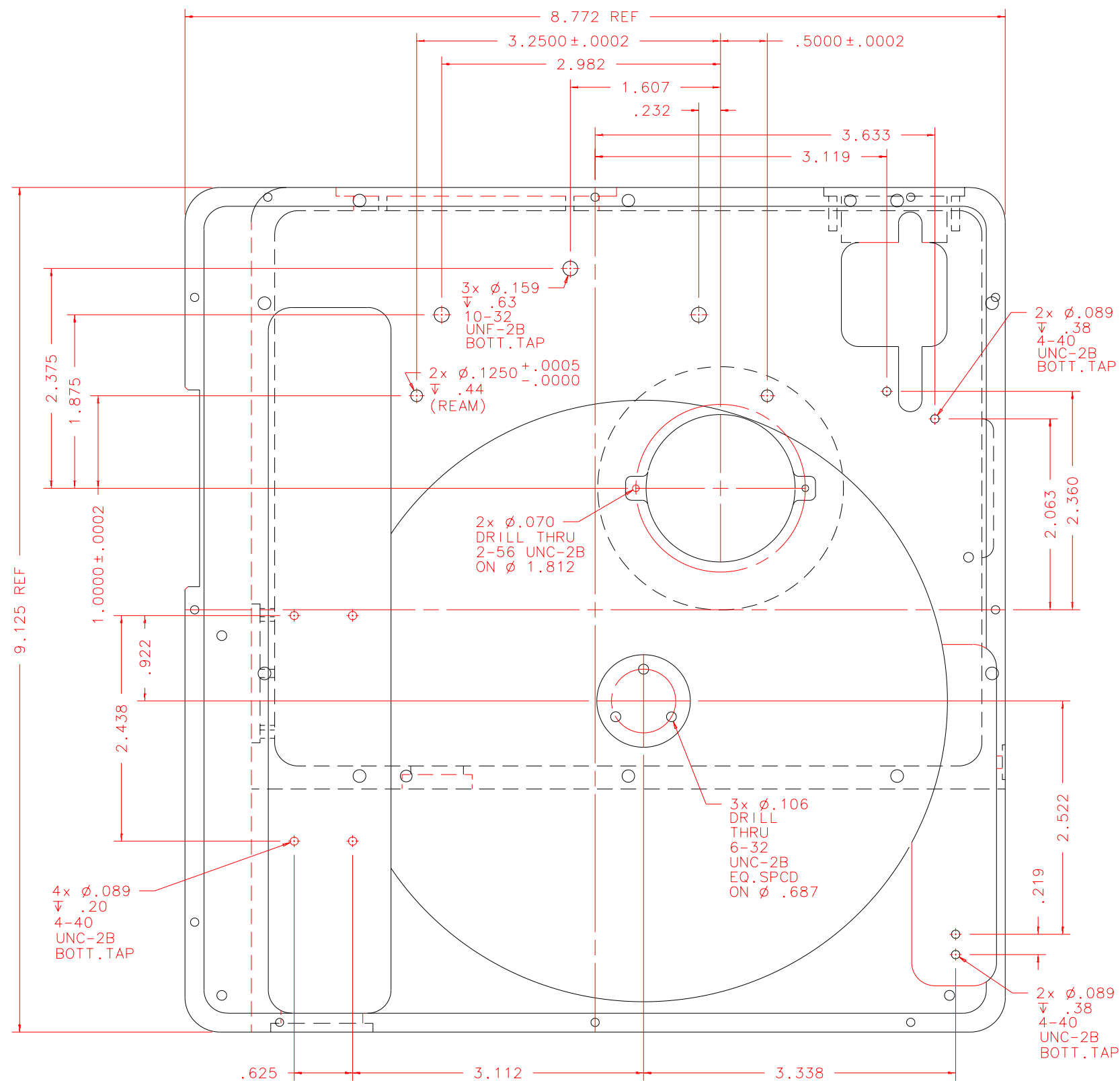
VIEW 13: SCALE 3/4 DUPLICATE OF FRONT VIEW SHEET 1
