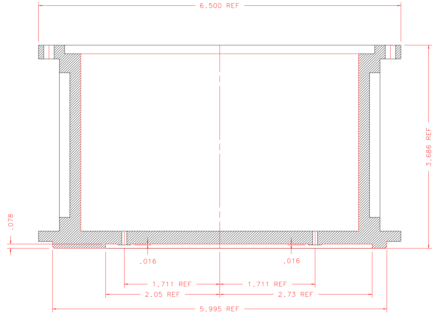
SECTION B-B: SCALE FULL
