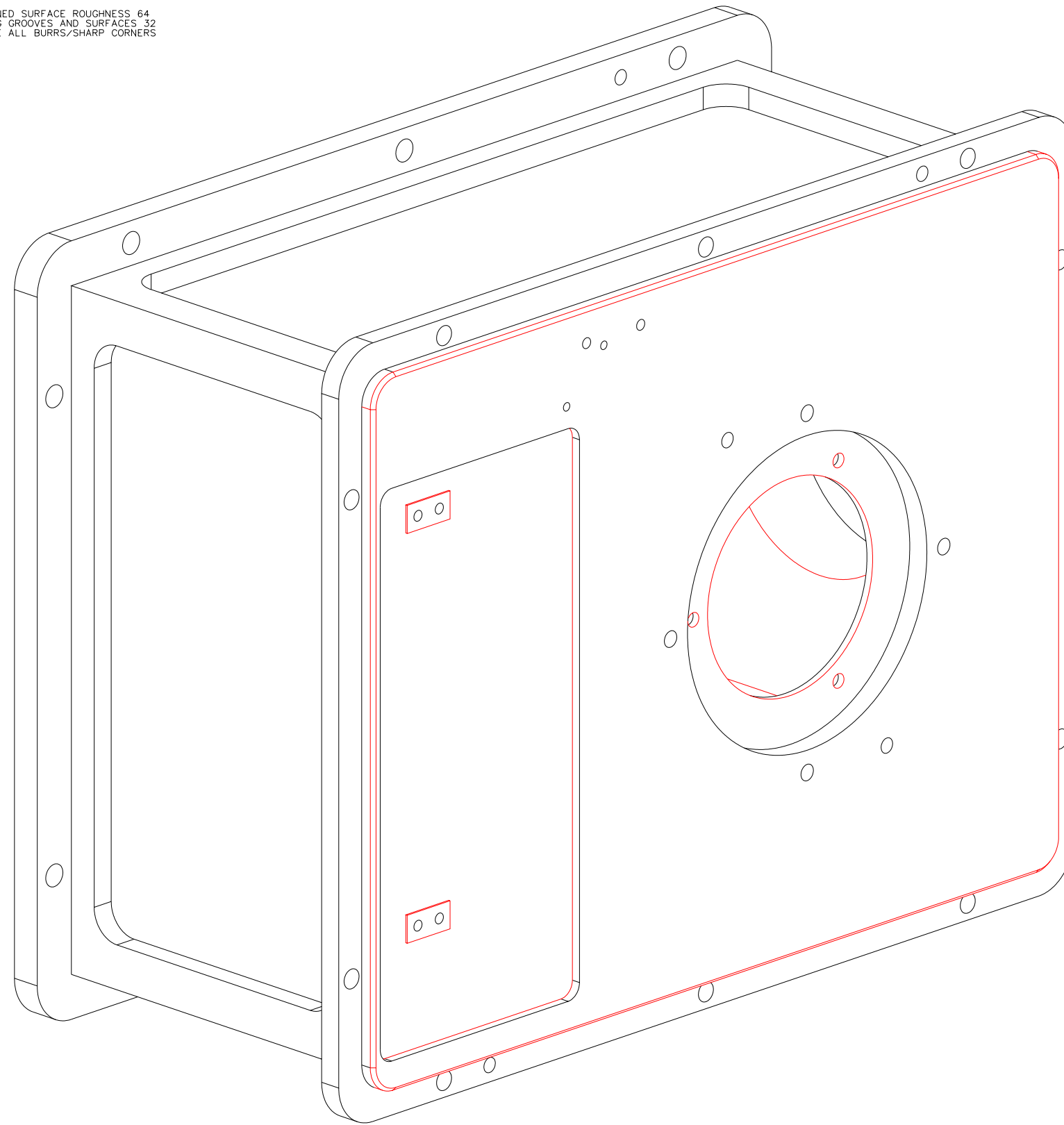
ISOVIEW 6: SCALE FULL
