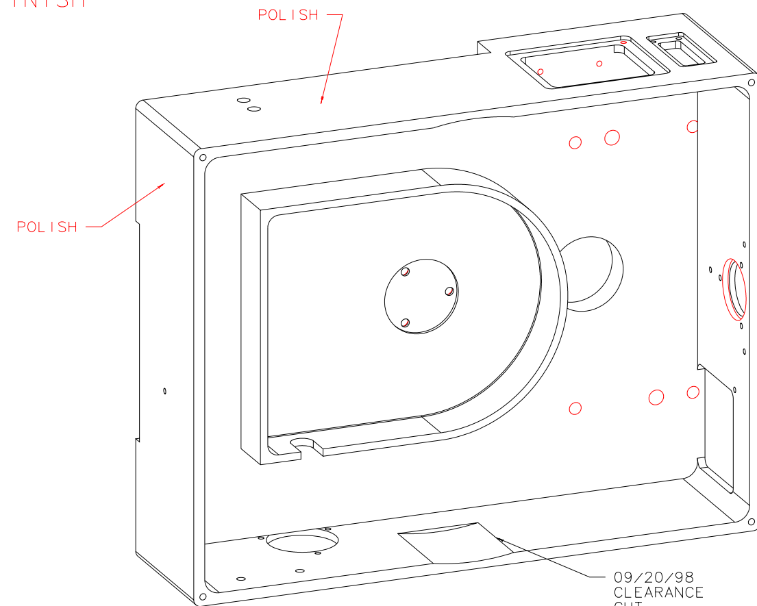
ISOVIEW 2: SCALE 1:2
